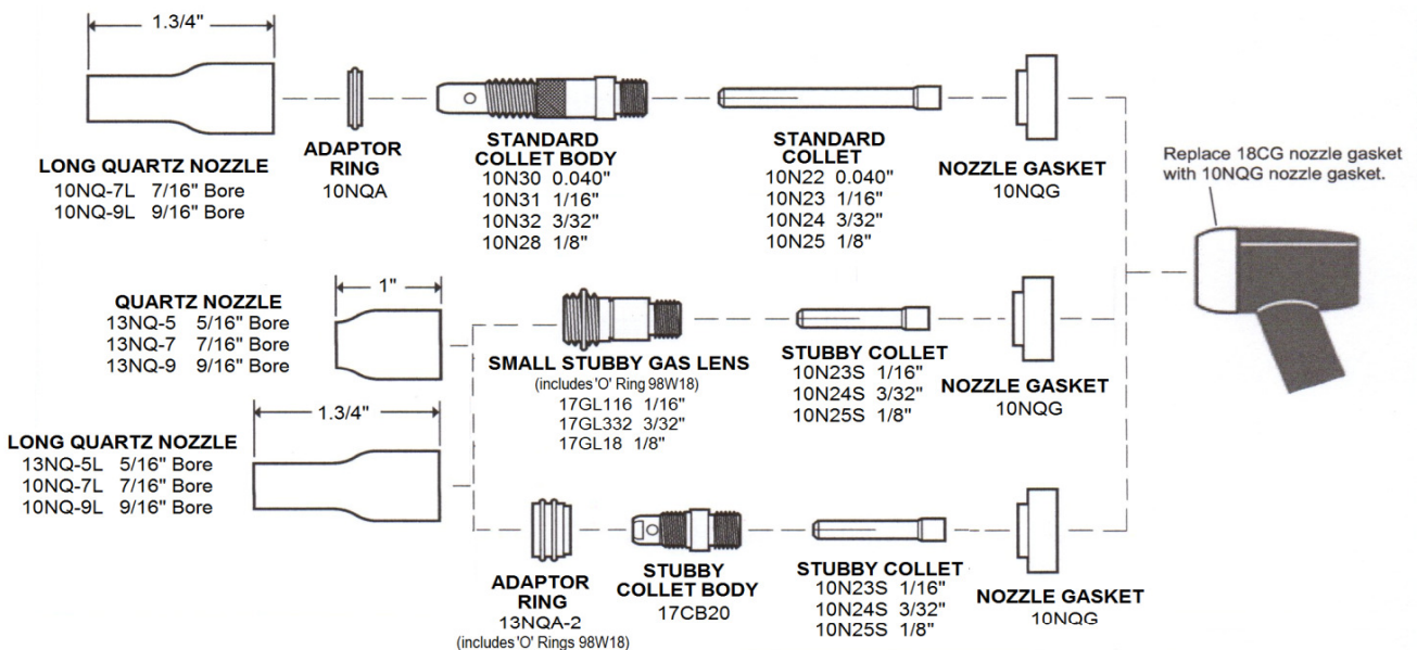
13NQ-7 7/16" BORE x 1" LONG
